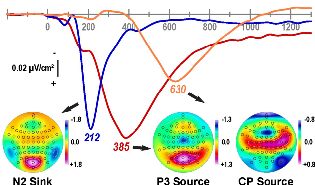
Figure 1. Factor loadings of the targeted three temporal PCA factors extracted from CSD waveforms ( N = 152 ; Kayser et al., 2016) and corresponding grand mean factor score topographies for the present sample ( N = 127 ). Factor labels reflect the peak latency [ms] of the factor loadings relative to stimulus onset.
